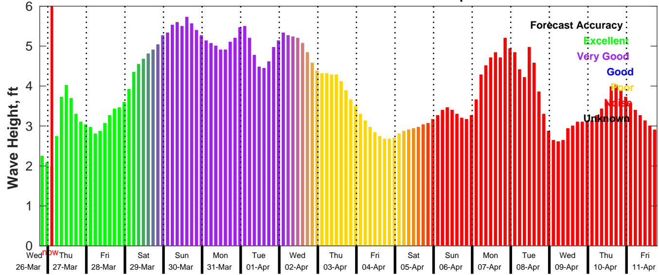
GFS Wave Forecast for NDBC 41004 from 26-Mar-2025 19:00:00 to 11-Apr-2025 19:00:00
