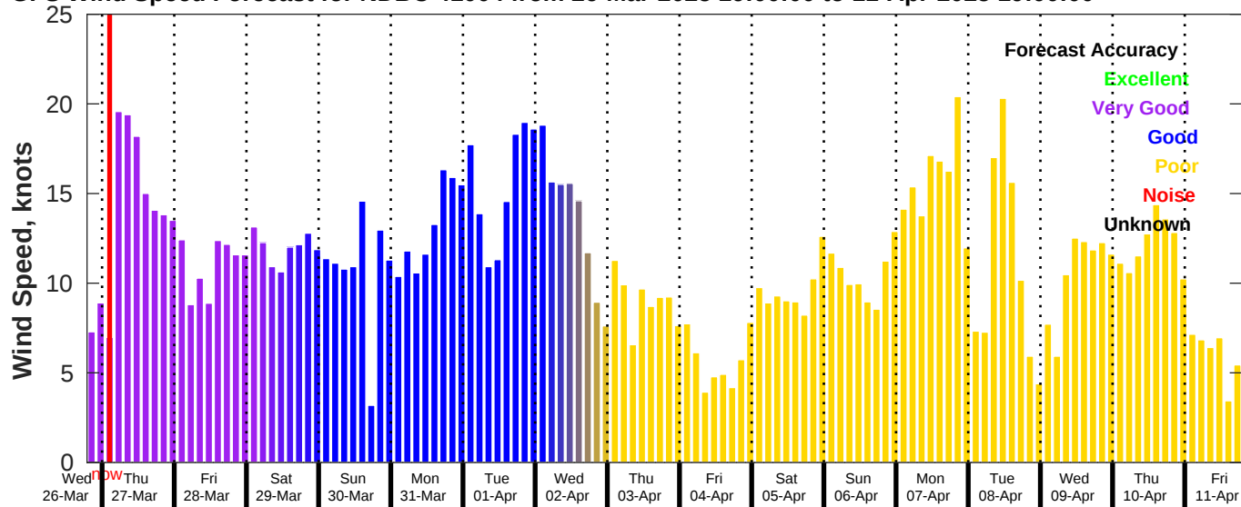
GFS Wind Speed Forecast for NDBC 41004 from 26-Mar-2025 19:00:00 to 11-Apr-2025 19:00:00
