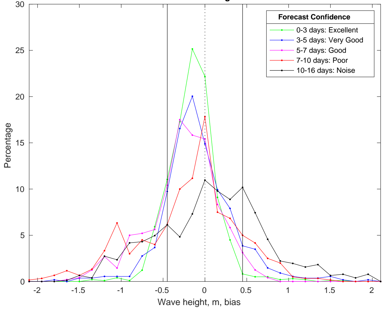
NDBC 41013 vs GFS Waves Bias Histogram: 27-Mar-2025
