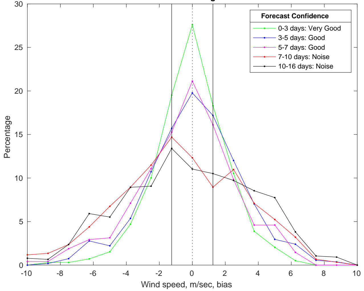
NDBC 41013 vs GFS Winds Bias Histogram: 27-Mar-2025
