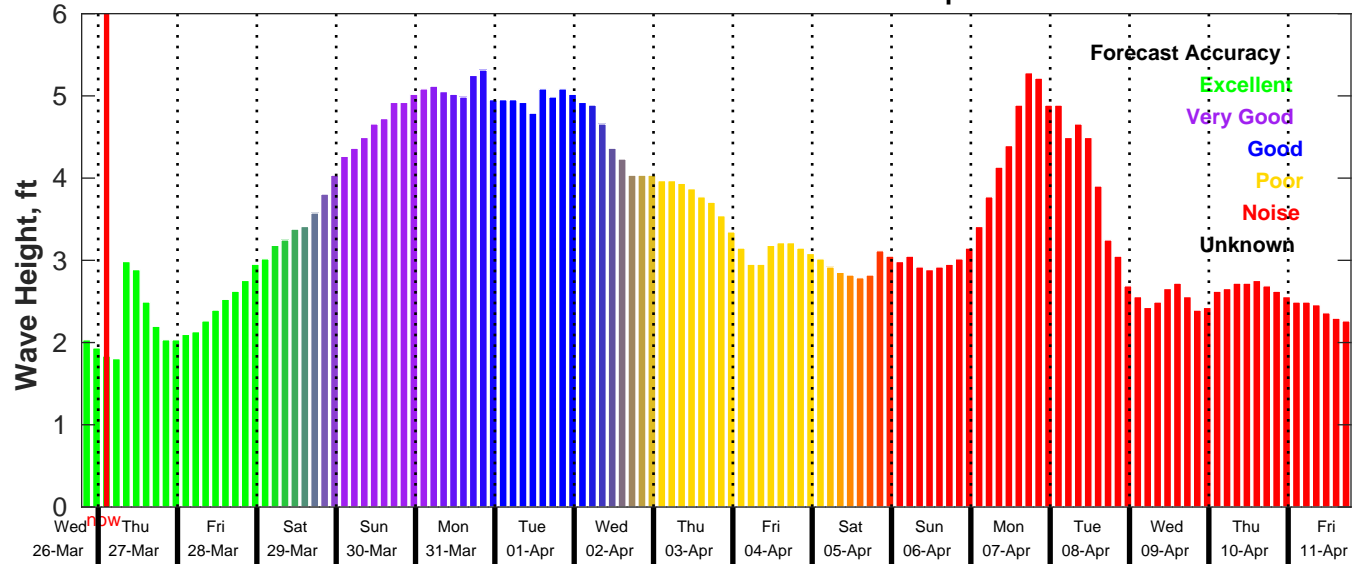
GFS Wave Forecast for NDBC 41013 from 26-Mar-2025 19:00:00 to 11-Apr-2025 19:00:00
