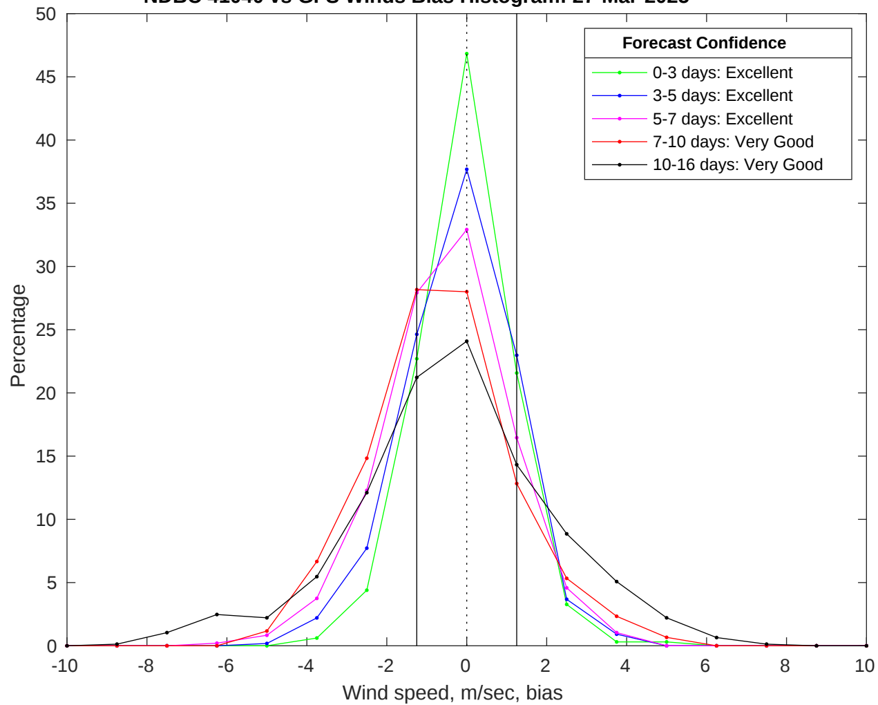
NDBC 41040 vs GFS Winds Bias Histogram: 27-Mar-2025
