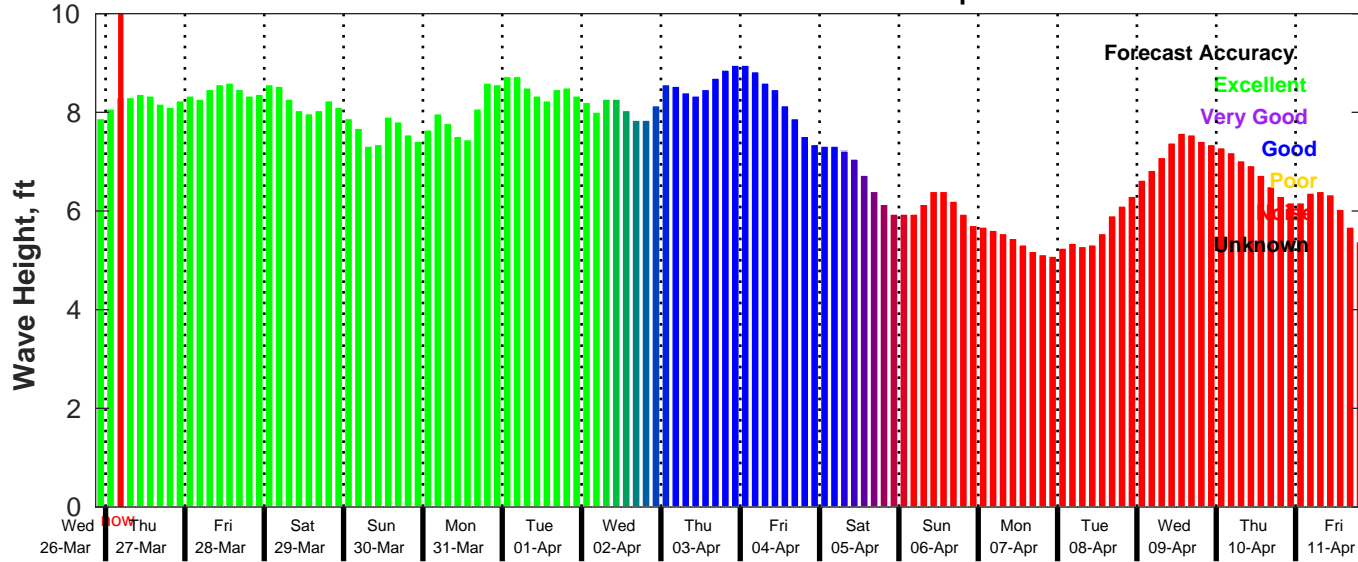
GFS Wave Forecast for NDBC 41040 from 26-Mar-2025 21:00:00 to 11-Apr-2025 21:00:00
