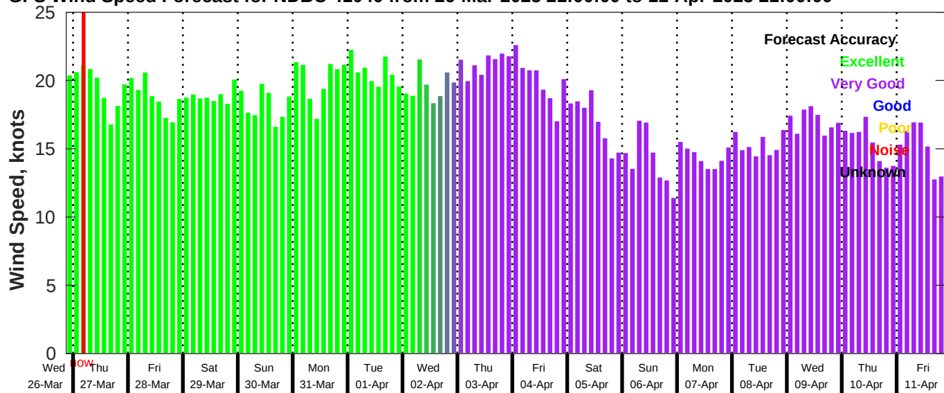
GFS Wind Speed Forecast for NDBC 41040 from 26-Mar-2025 21:00:00 to 11-Apr-2025 21:00:00
