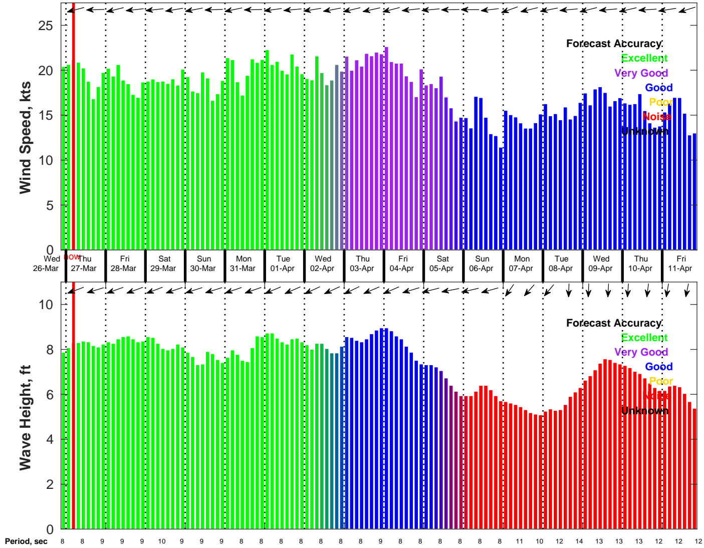
Wind & Wave Forecast for NDBC 41040 from 26-Mar-2025 21:00:00 to 11-Apr-2025 21:00:00
