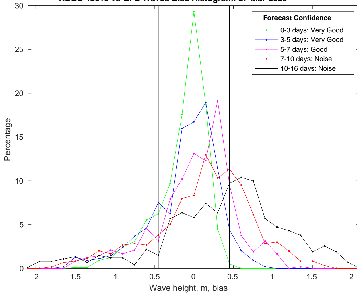
NDBC 42019 vs GFS Waves Bias Histogram: 27-Mar-2025
