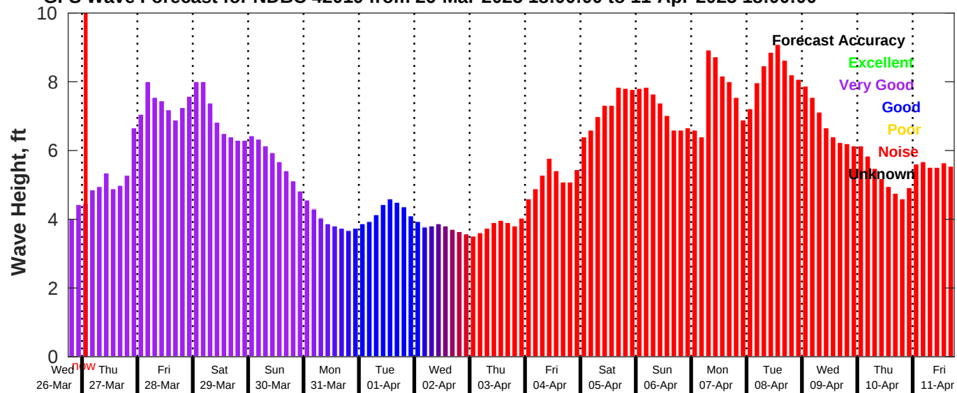
GFS Wave Forecast for NDBC 42019 from 26-Mar-2025 18:00:00 to 11-Apr-2025 18:00:00
