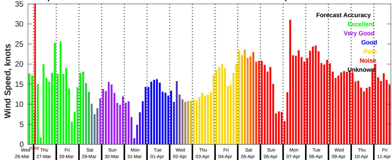
GFS Wind Speed Forecast for NDBC 42019 from 26-Mar-2025 18:00:00 to 11-Apr-2025 18:00:00
