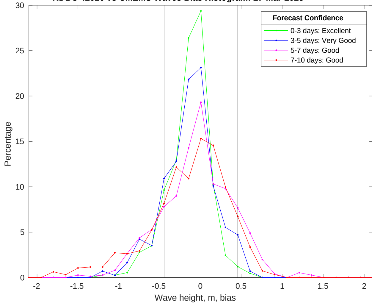
NDBC 42020 vs CMEMS Waves Bias Histogram: 27-Mar-2025
