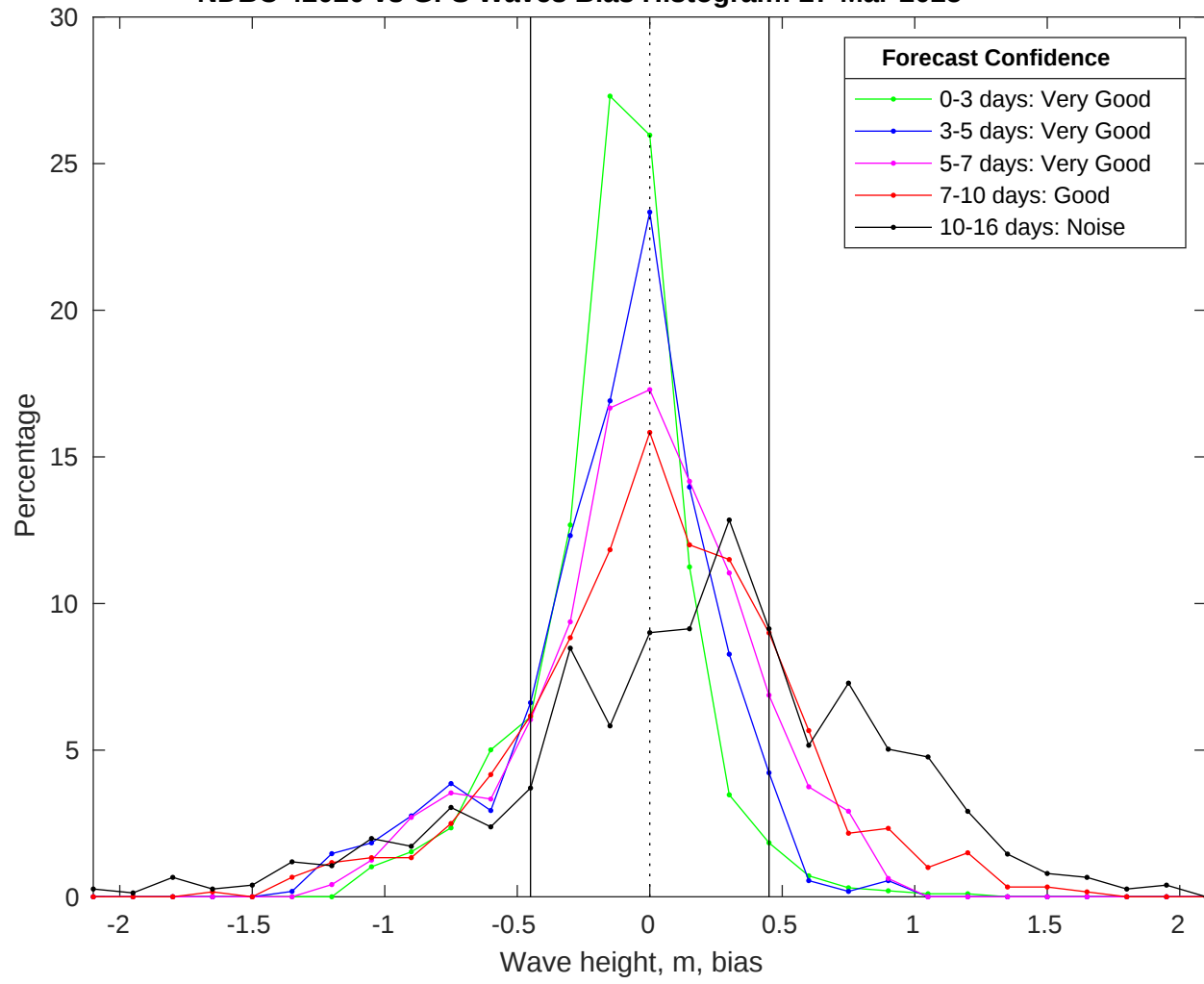
NDBC 42020 vs GFS Waves Bias Histogram: 27-Mar-2025
