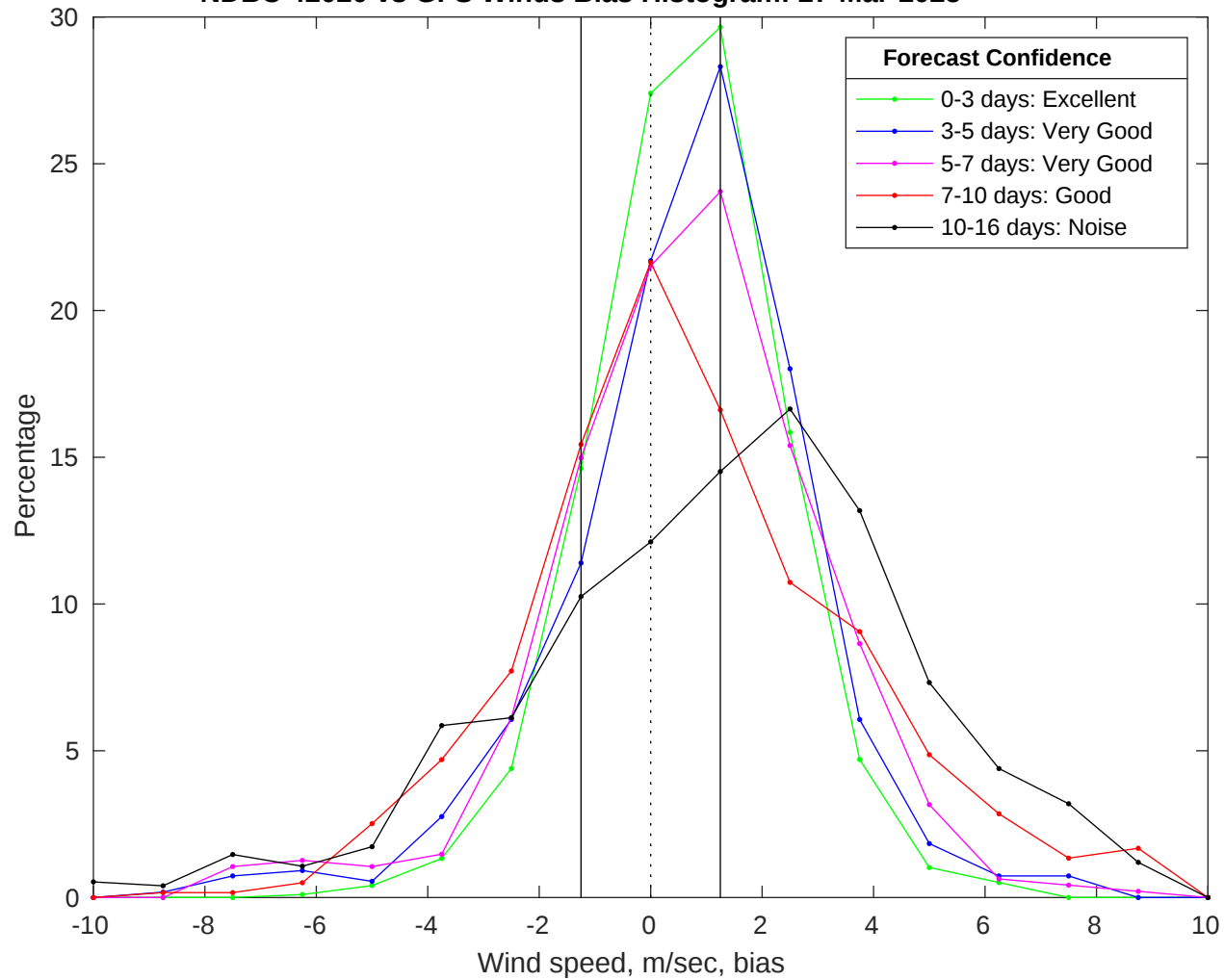
NDBC 42020 vs GFS Winds Bias Histogram: 27-Mar-2025
