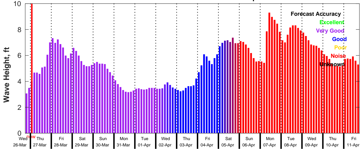
GFS Wave Forecast for NDBC 42020 from 26-Mar-2025 18:00:00 to 11-Apr-2025 18:00:00
