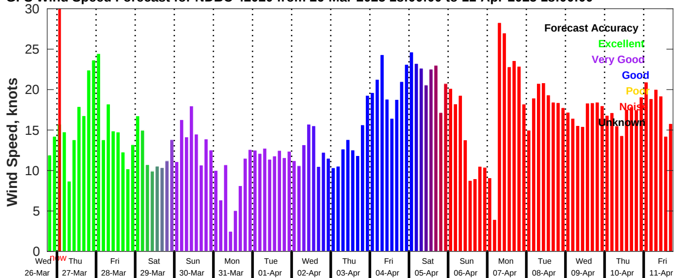
GFS Wind Speed Forecast for NDBC 42020 from 26-Mar-2025 18:00:00 to 11-Apr-2025 18:00:00
