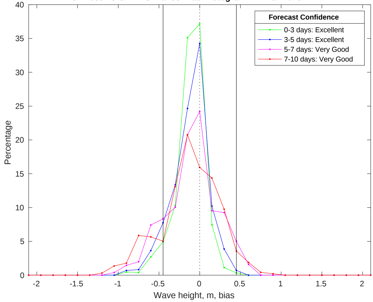
NDBC 42035 vs CMEMS Waves Bias Histogram: 27-Mar-2025
