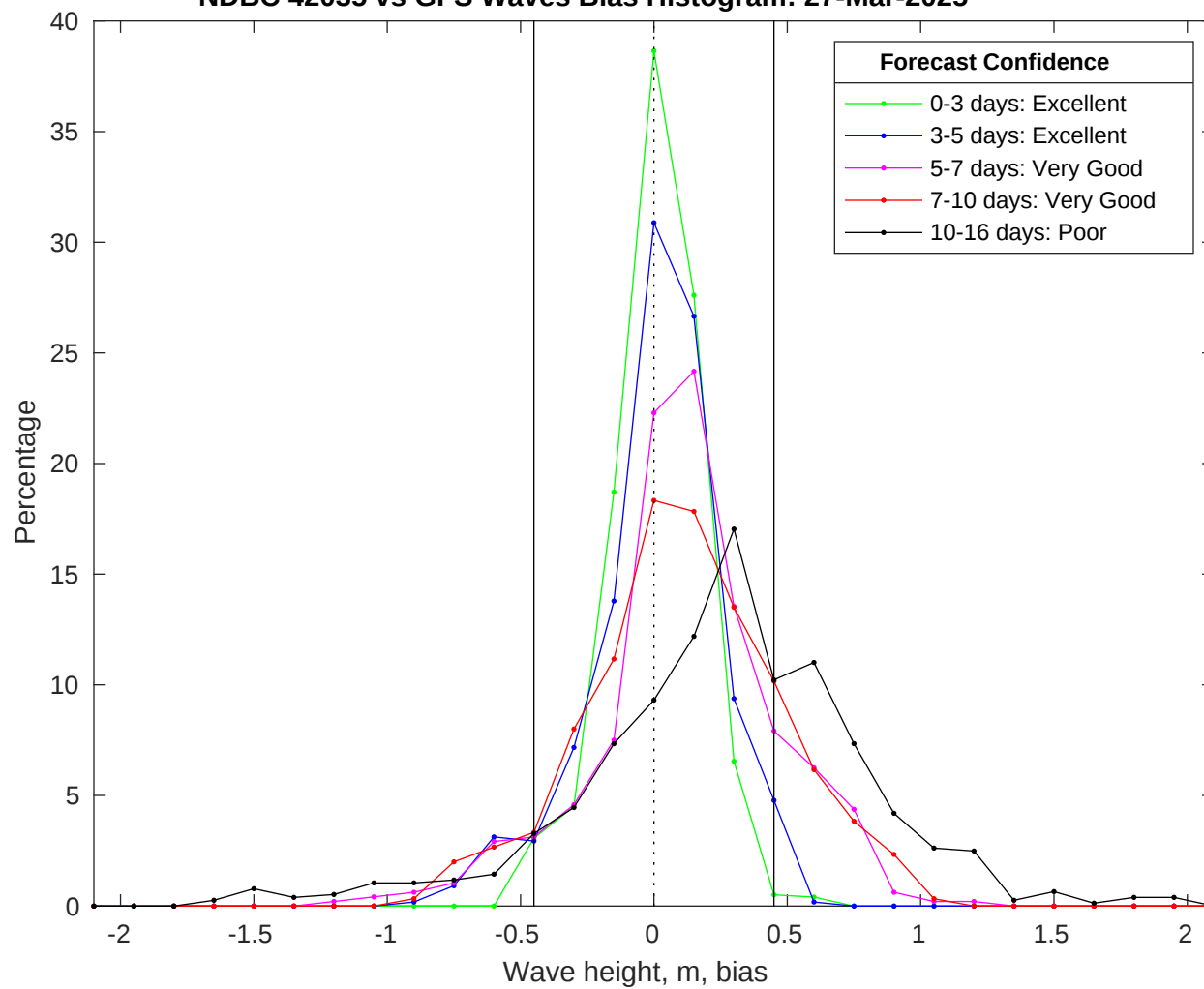
NDBC 42035 vs GFS Waves Bias Histogram: 27-Mar-2025
