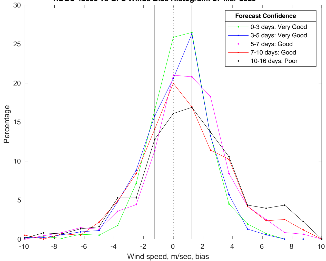
NDBC 42035 vs GFS Winds Bias Histogram: 27-Mar-2025
