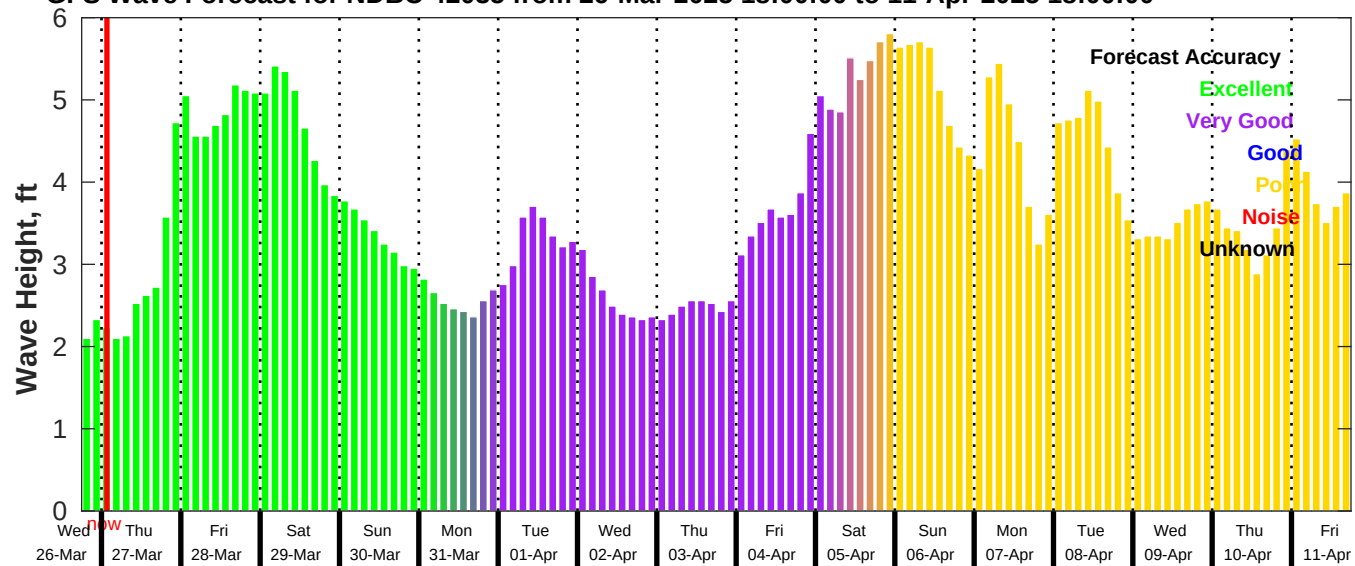
GFS Wave Forecast for NDBC 42035 from 26-Mar-2025 18:00:00 to 11-Apr-2025 18:00:00
