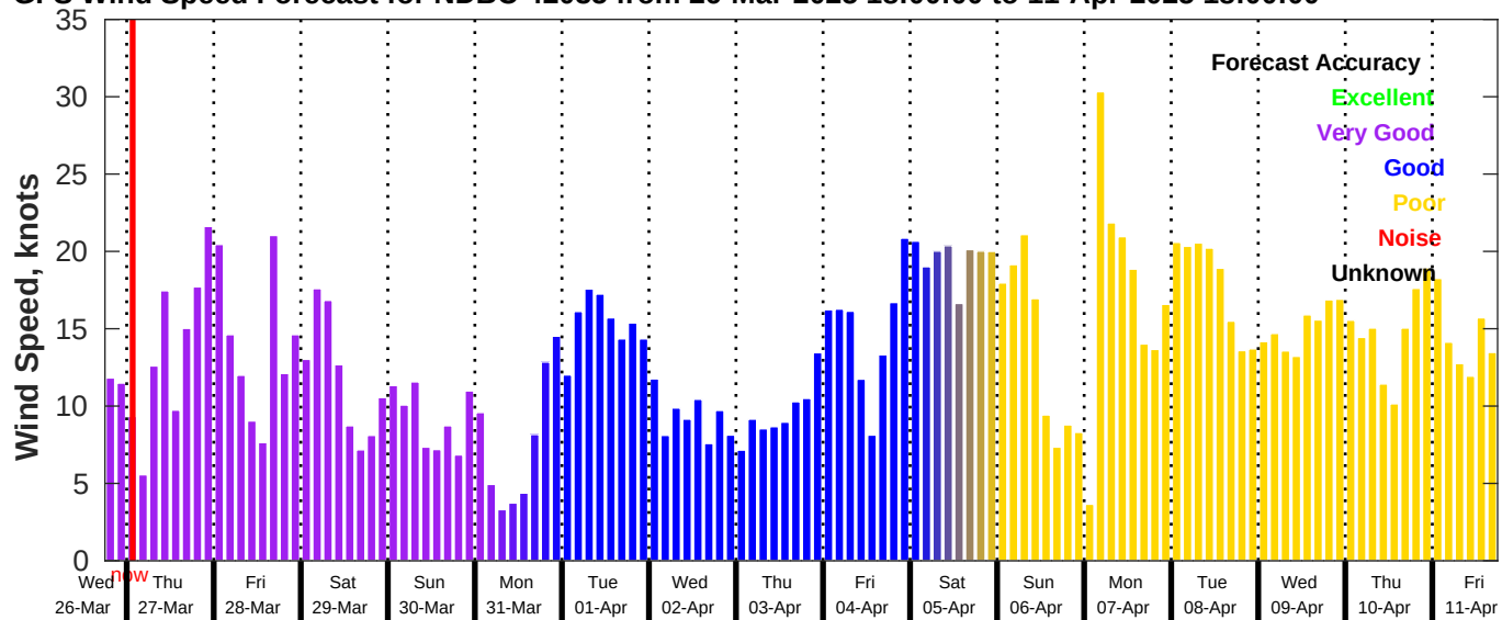
GFS Wind Speed Forecast for NDBC 42035 from 26-Mar-2025 18:00:00 to 11-Apr-2025 18:00:00
