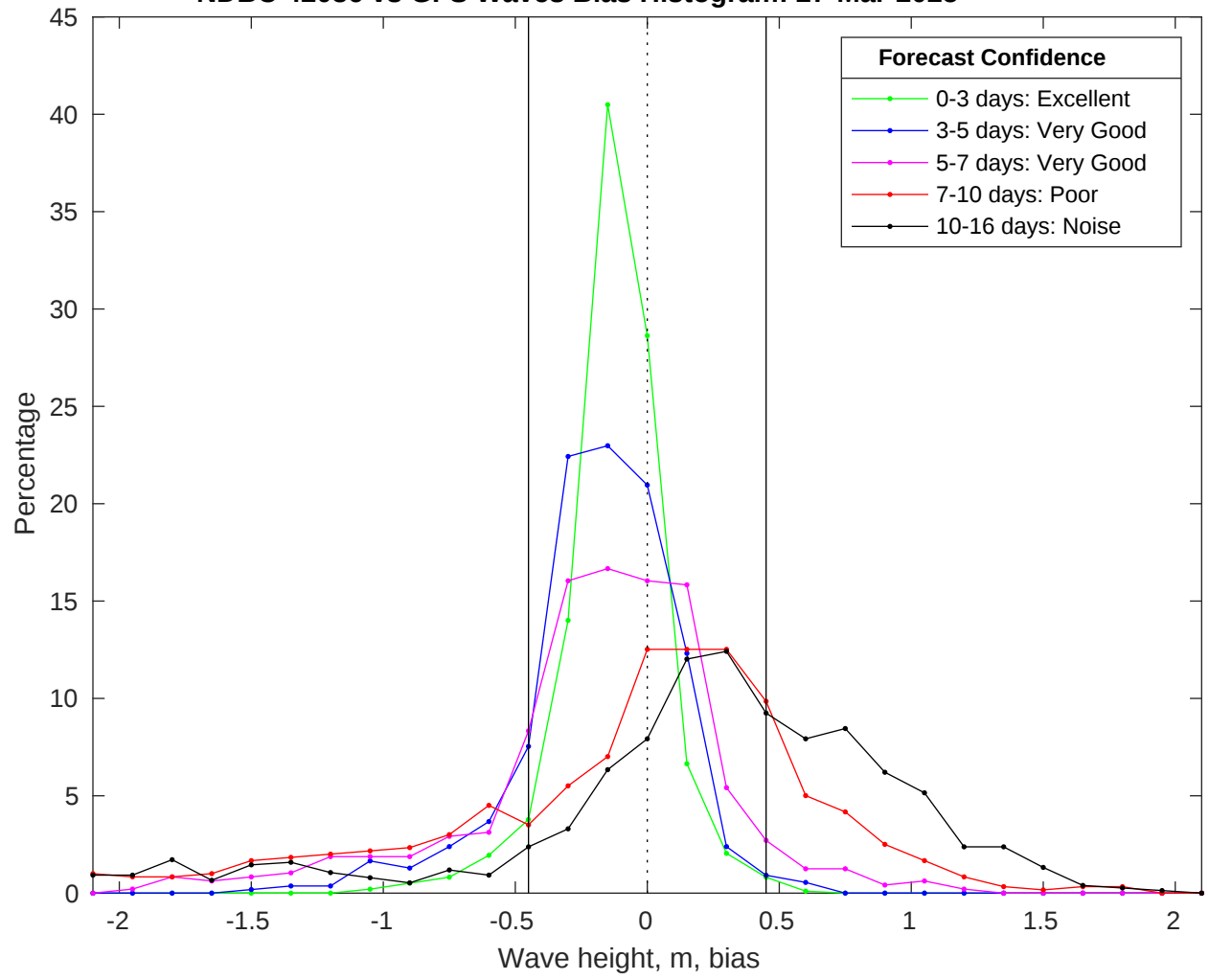
NDBC 42036 vs GFS Waves Bias Histogram: 27-Mar-2025
