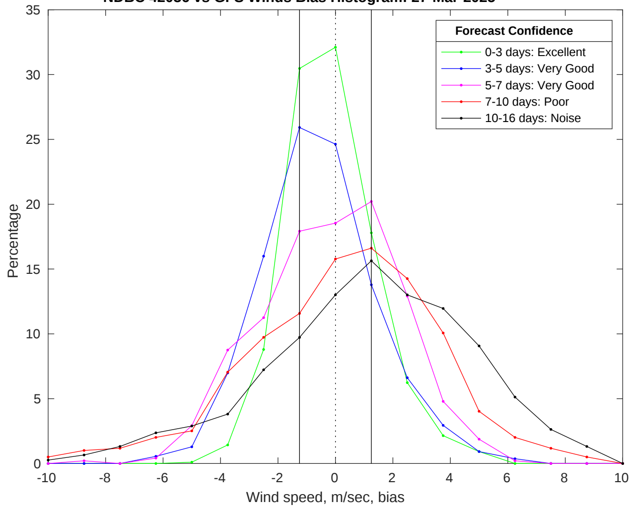
NDBC 42036 vs GFS Winds Bias Histogram: 27-Mar-2025
