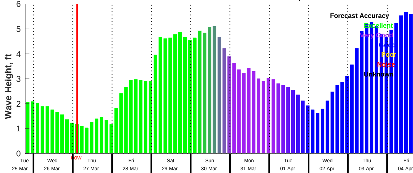
CMEMS Wave Forecast for NDBC 42036 from 25-Mar-2025 19:00:00 to 04-Apr-2025 19:00:00
