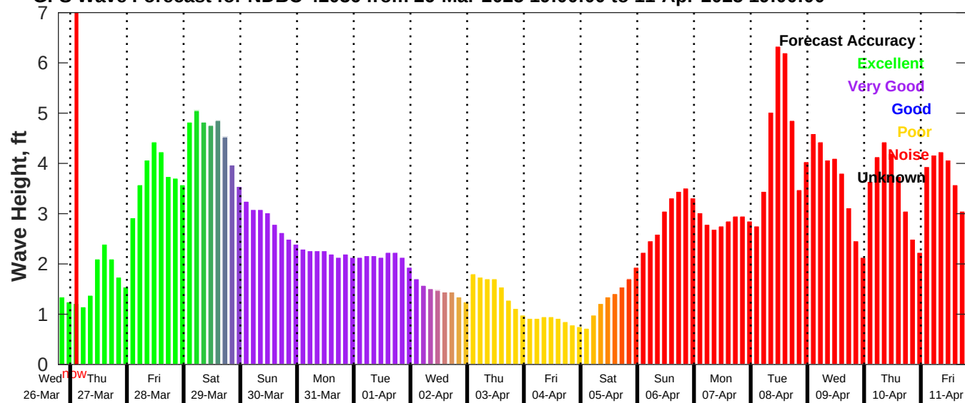
GFS Wave Forecast for NDBC 42036 from 26-Mar-2025 19:00:00 to 11-Apr-2025 19:00:00
