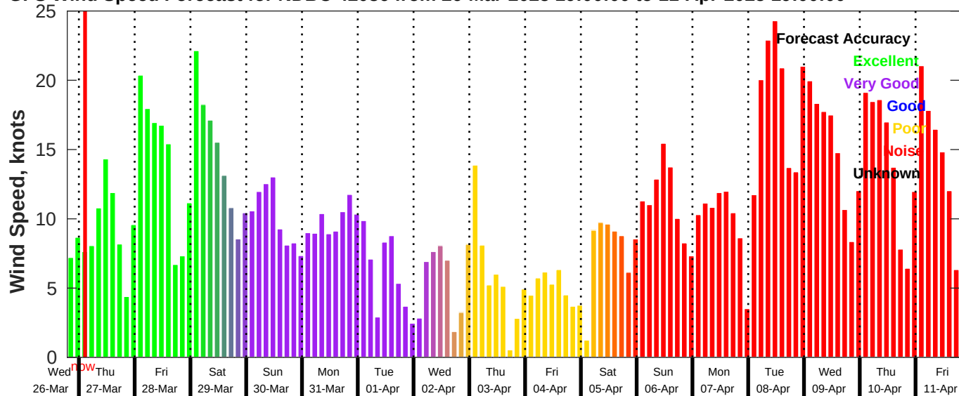
GFS Wind Speed Forecast for NDBC 42036 from 26-Mar-2025 19:00:00 to 11-Apr-2025 19:00:00
