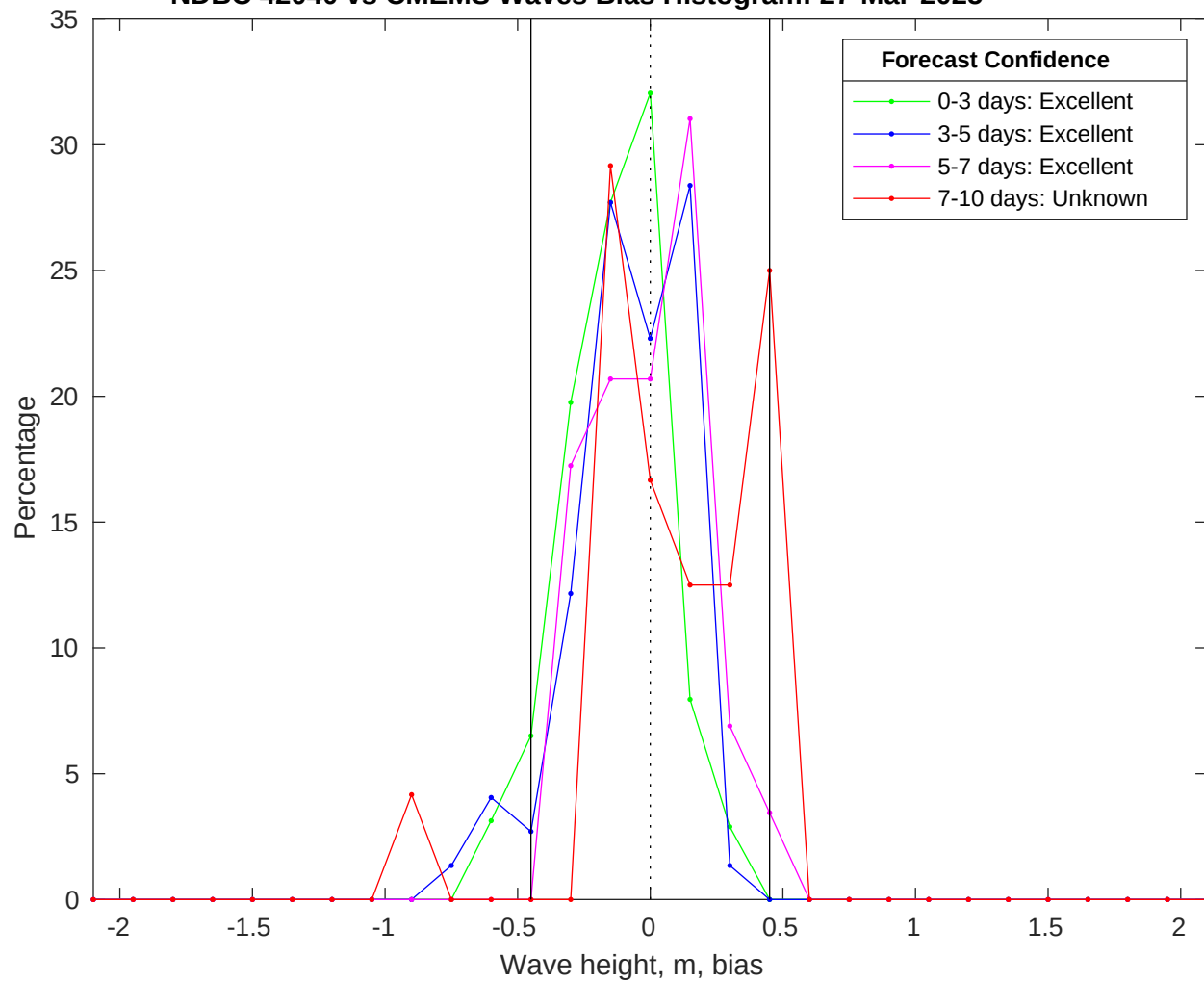
NDBC 42040 vs CMEMS Waves Bias Histogram: 27-Mar-2025
