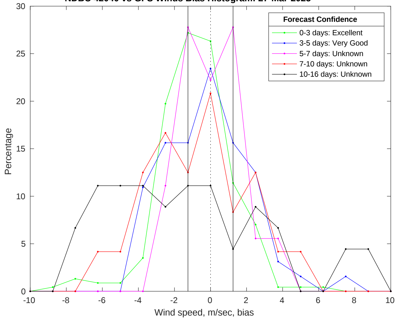
NDBC 42040 vs GFS Winds Bias Histogram: 27-Mar-2025
