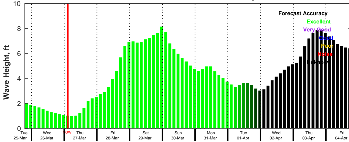
CMEMS Wave Forecast for NDBC 42040 from 25-Mar-2025 19:00:00 to 04-Apr-2025 19:00:00
