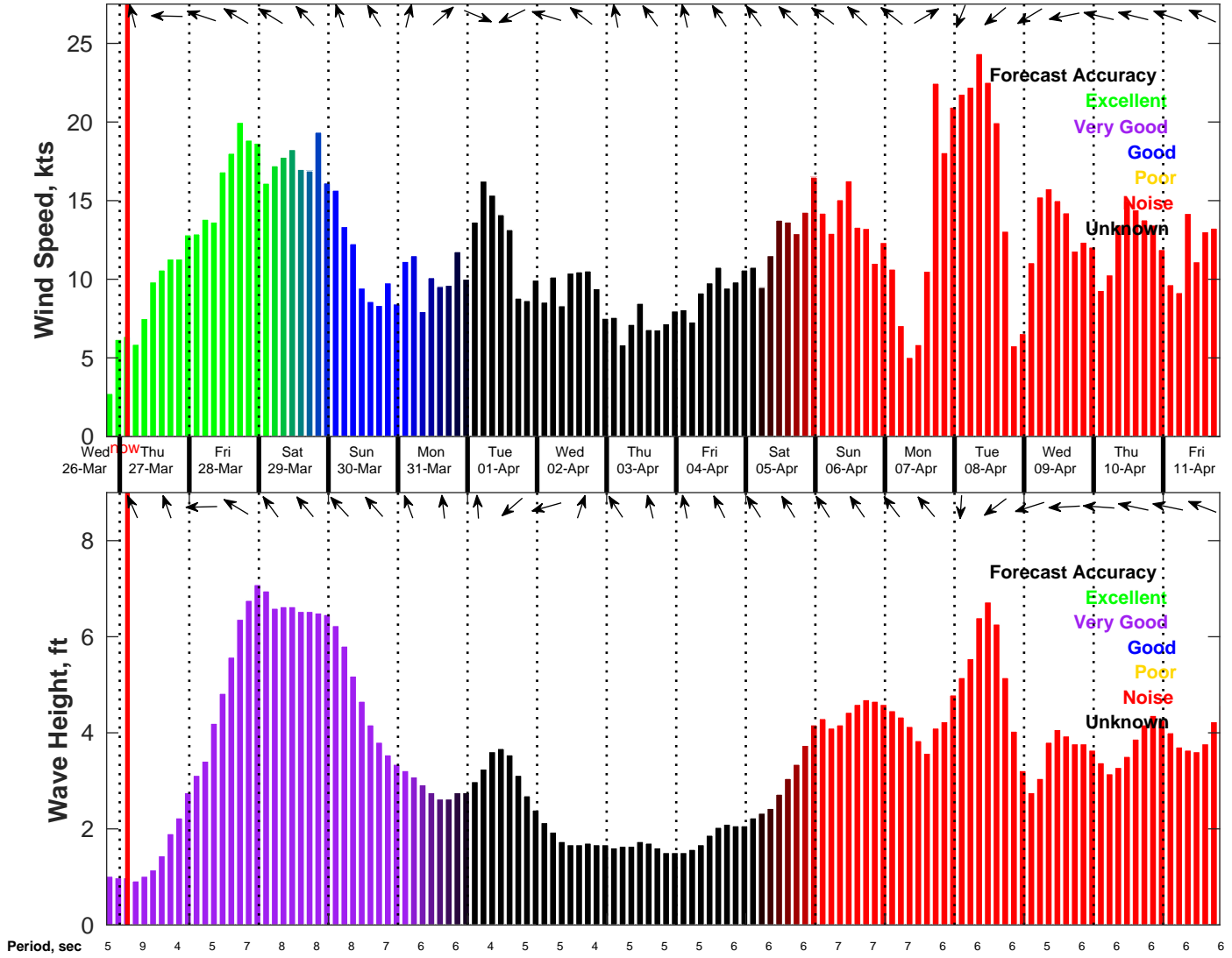
Wind & Wave Forecast for NDBC 42040 from 26-Mar-2025 19:00:00 to 11-Apr-2025 19:00:00
