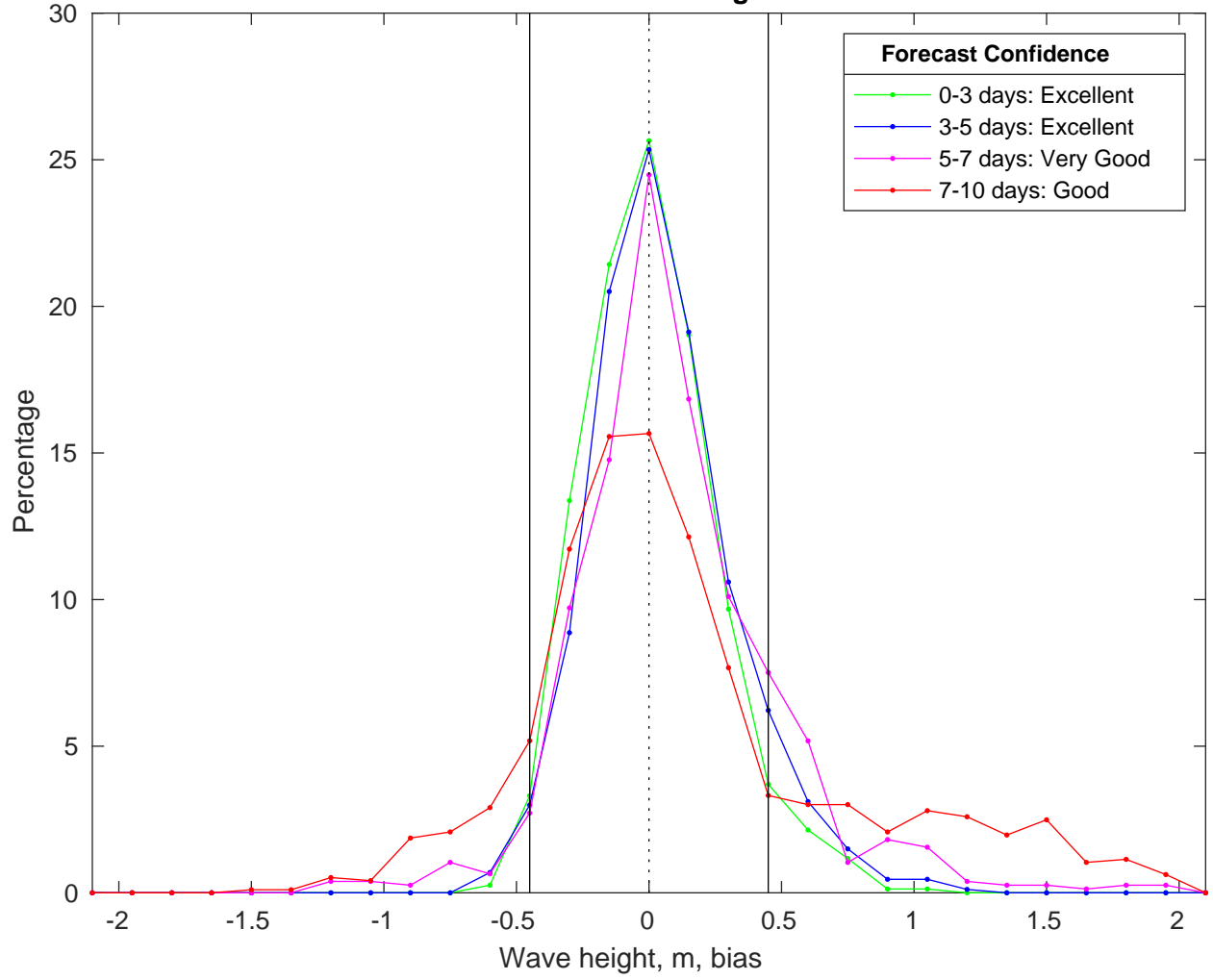
NDBC 46011 vs CMEMS Waves Bias Histogram: 27-Mar-2025
