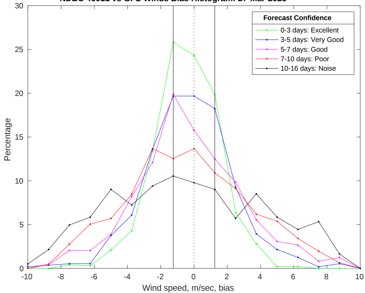
NDBC 46011 vs GFS Winds Bias Histogram: 27-Mar-2025
