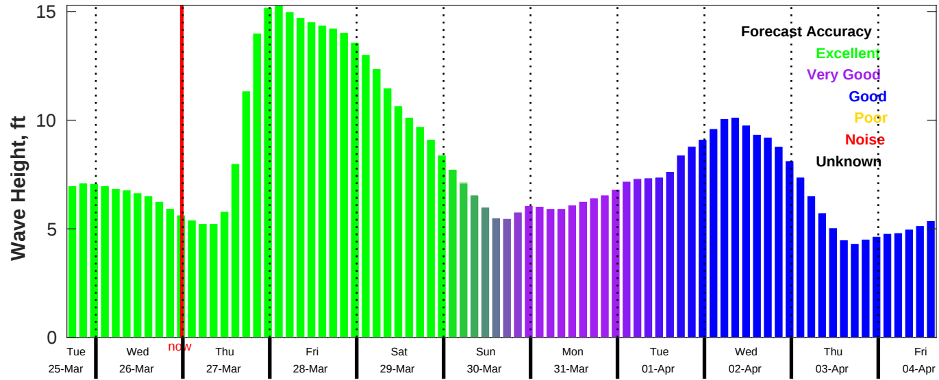
CEMS Wave Forecast for NDBC 46011 from 25-Mar-2025 16:00:00 to 04-Apr-2025 16:00:00
