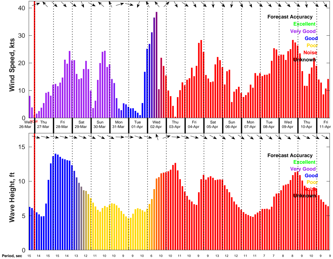
Wind & Wave Forecast for NDBC 46011 from 26-Mar-2025 16:00:00 to 11-Apr-2025 16:00:00
