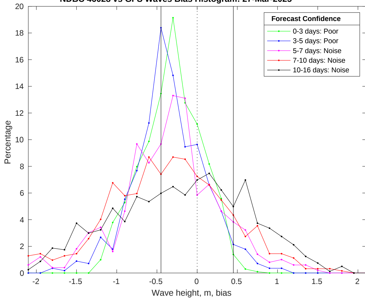
NDBC 46028 vs GFS Waves Bias Histogram: 27-Mar-2025
