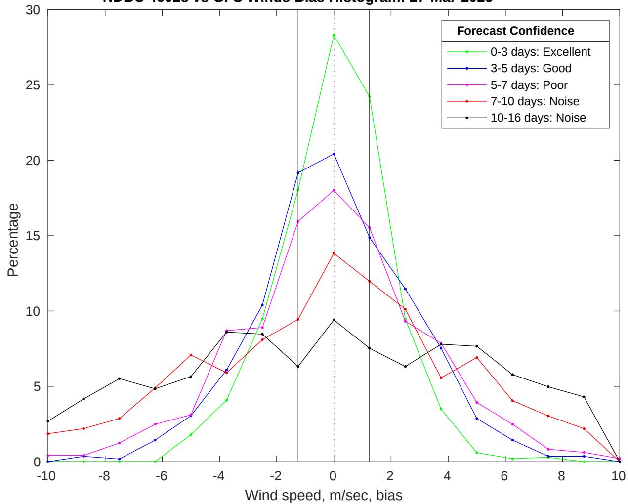
NDBC 46028 vs GFS Winds Bias Histogram: 27-Mar-2025
