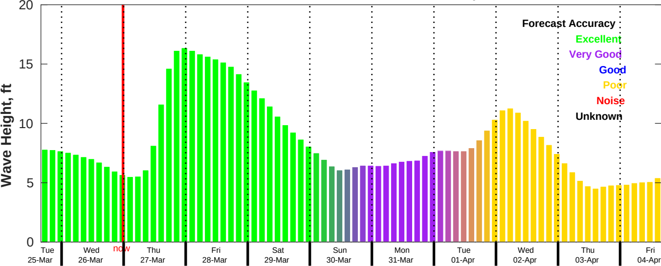
CMEMS Wave Forecast for NDBC 46028 from 25-Mar-2025 16:00:00 to 04-Apr-2025 16:00:00
