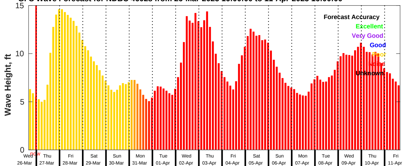
GFS Wave Forecast for NDBC 46028 from 26-Mar-2025 16:00:00 to 11-Apr-2025 16:00:00
