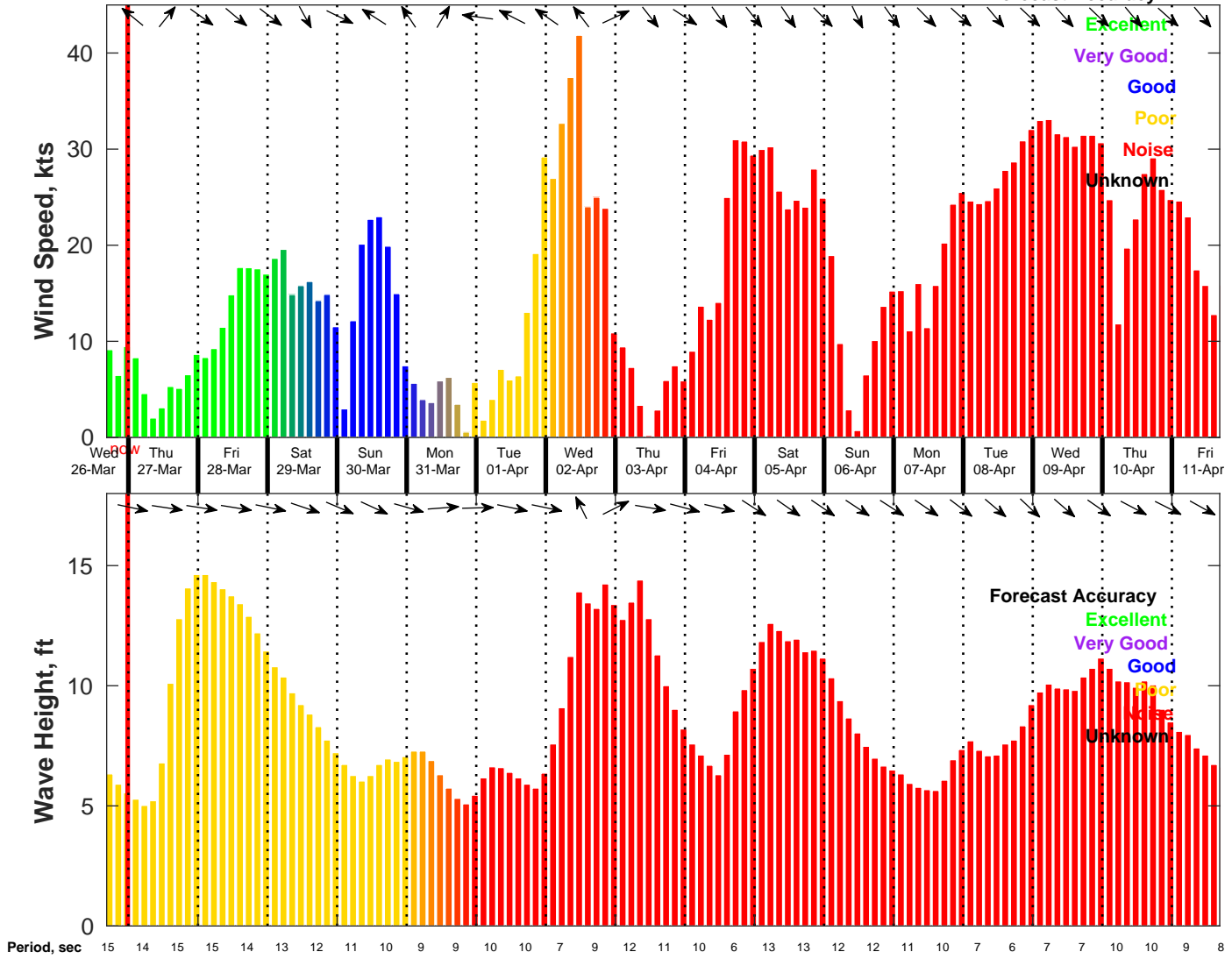
Wind & Wave Forecast for NDBC 46028 from 26-Mar-2025 16:00:00 to 11-Apr-2025 16:00:00
