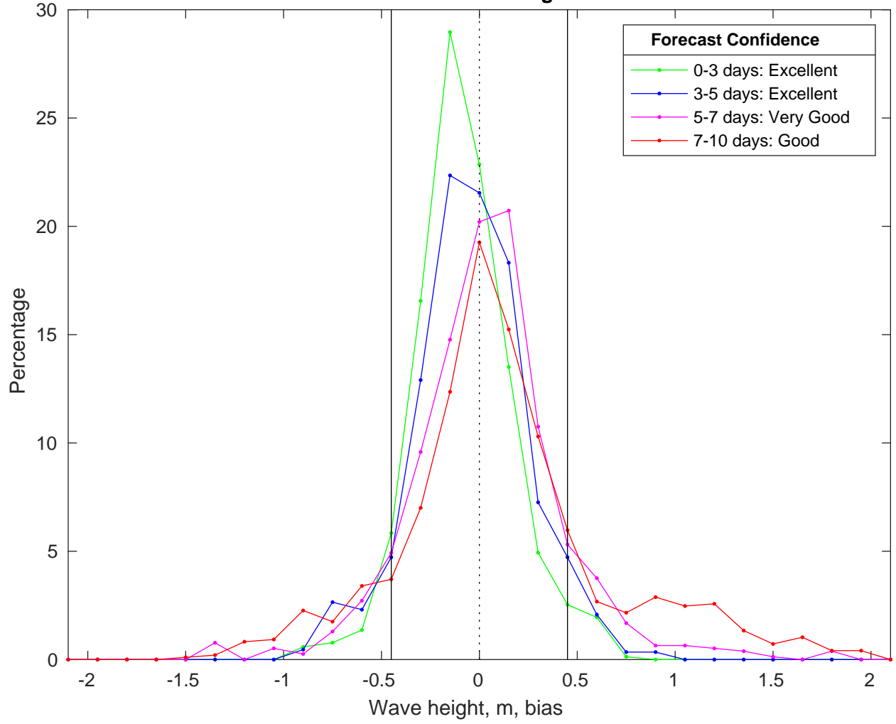
NDBC 46054 vs CMEMS Waves Bias Histogram: 27-Mar-2025
