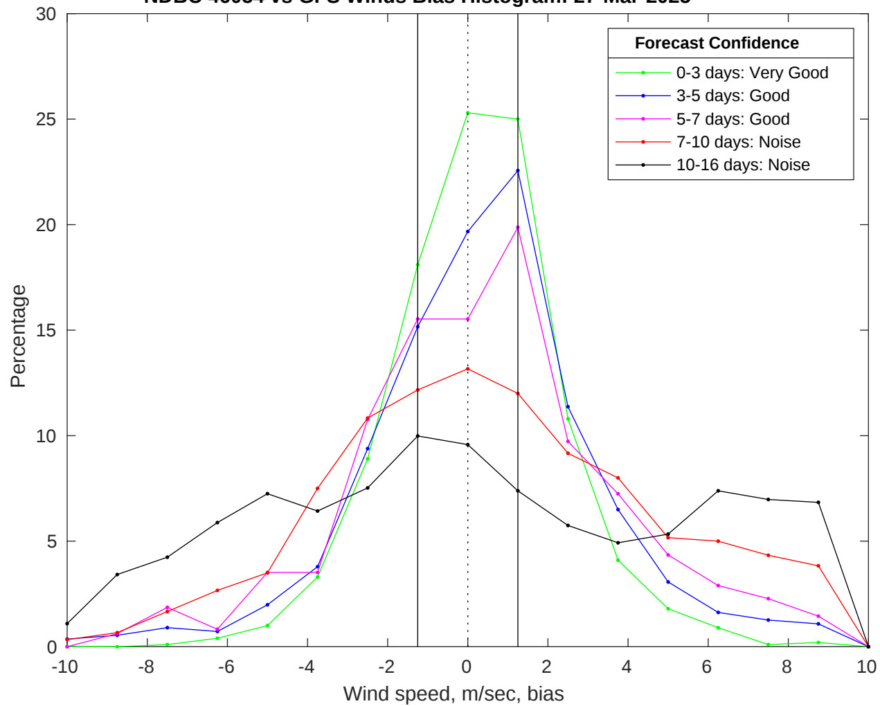
NDBC 46054 vs GFS Winds Bias Histogram: 27-Mar-2025
