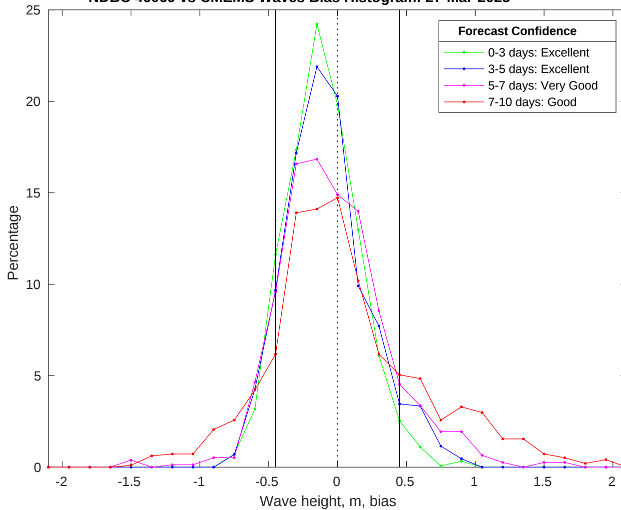
NDBC 46069 vs CMEMS Waves Bias Histogram: 27-Mar-2025
