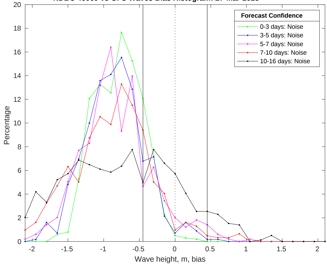
NDBC 46069 vs GFS Waves Bias Histogram: 27-Mar-2025
