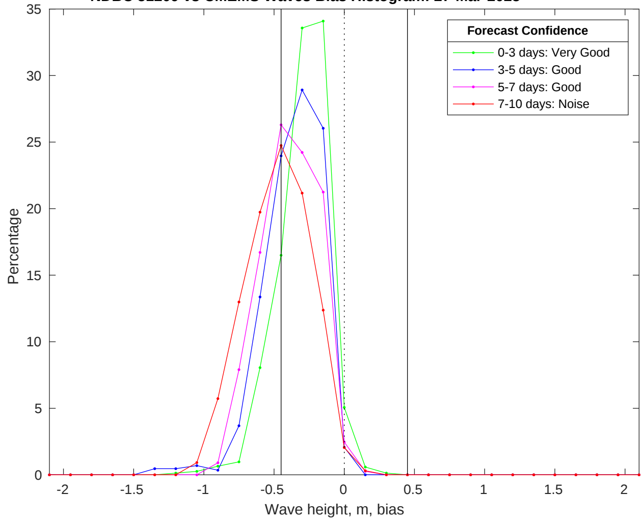
NDBC 51209 vs CMEMS Waves Bias Histogram: 27-Mar-2025
