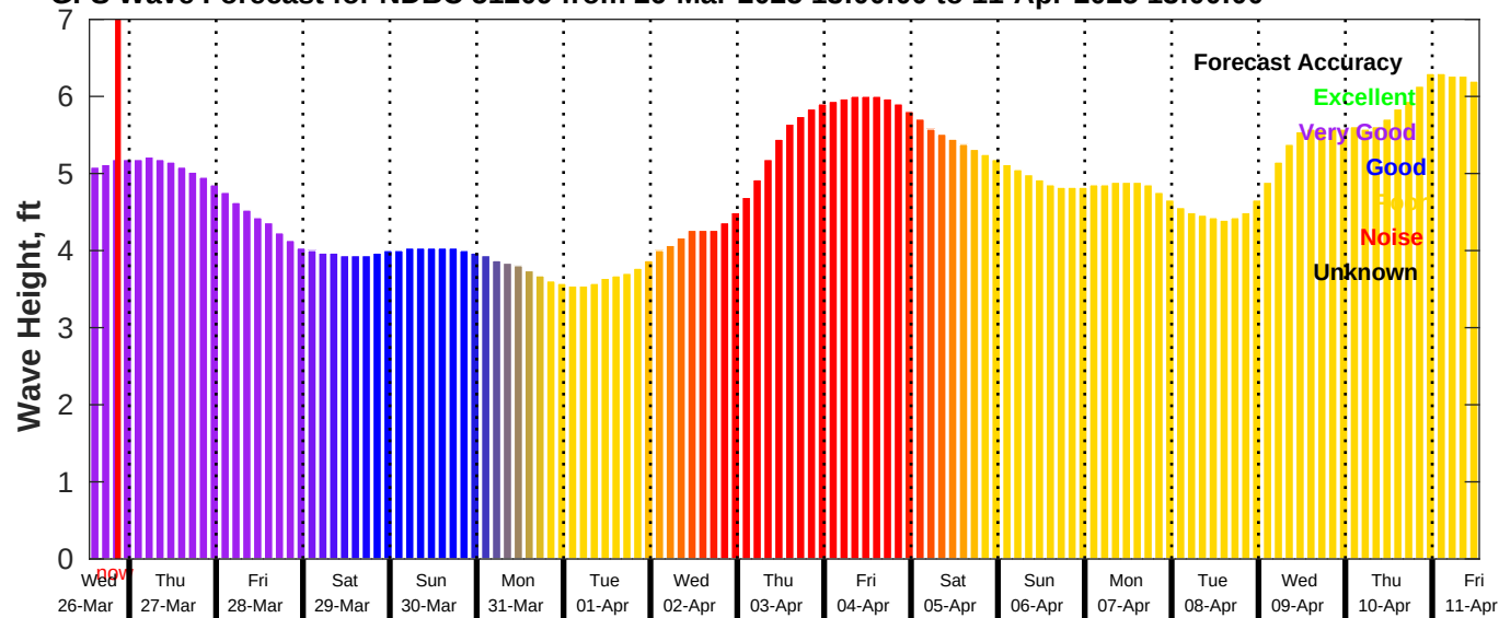
GFS Wave Forecast for NDBC 51209 from 26-Mar-2025 13:00:00 to 11-Apr-2025 13:00:00
