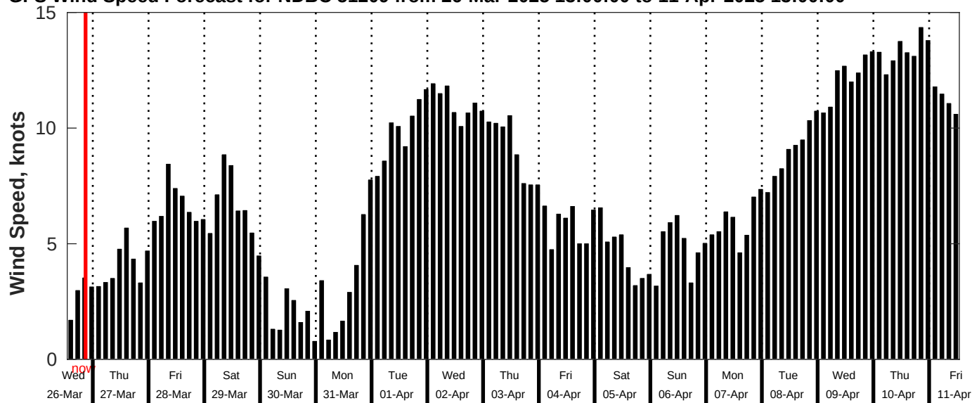
GFS Wind Speed Forecast for NDBC 51209 from 26-Mar-2025 13:00:00 to 11-Apr-2025 13:00:00
