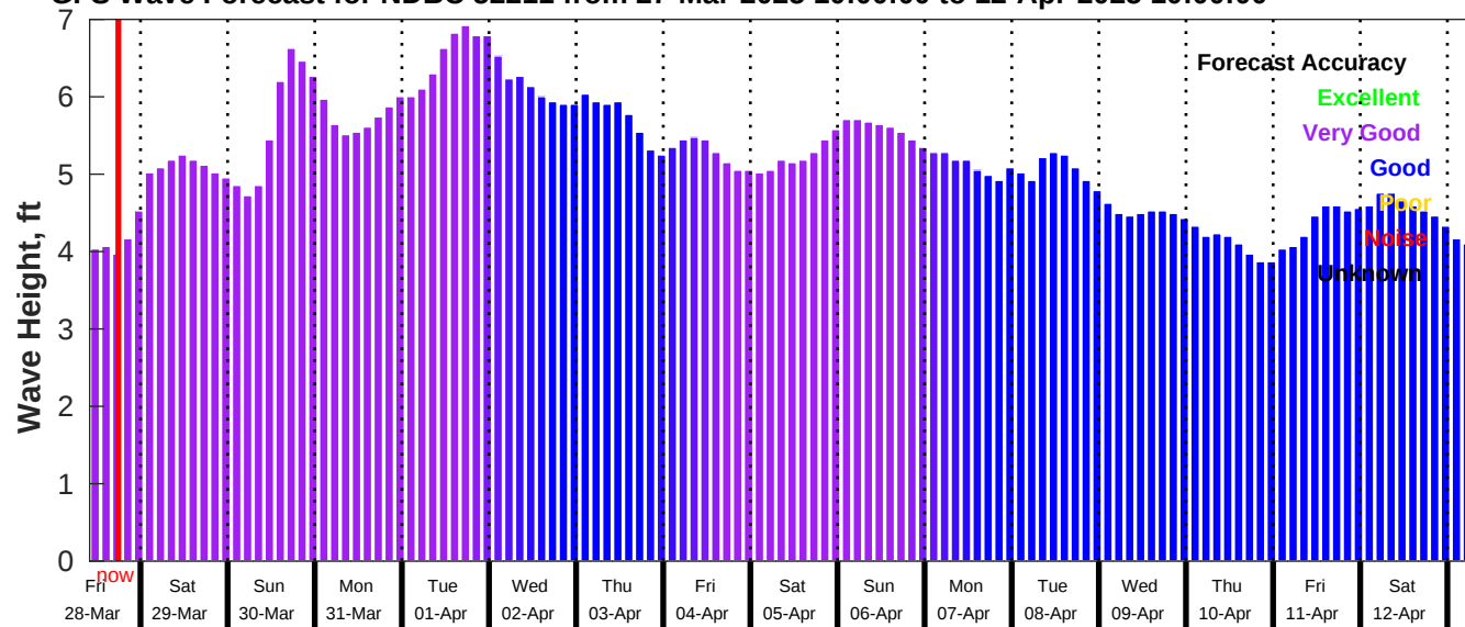
GFS Wave Forecast for NDBC 52211 from 27-Mar-2025 10:00:00 to 12-Apr-2025 10:00:00
