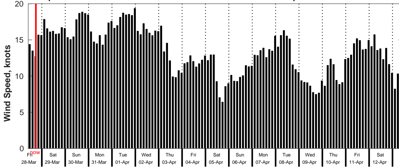
GFS Wind Speed Forecast for NDBC 52211 from 27-Mar-2025 10:00:00 to 12-Apr-2025 10:00:00
