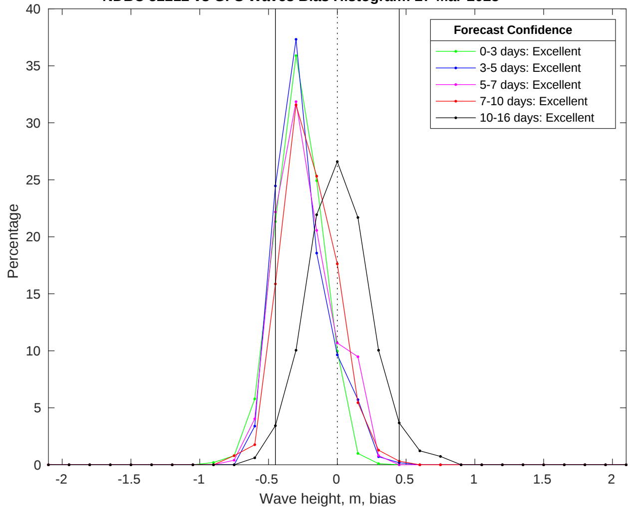
NDBC 52212 vs GFS Waves Bias Histogram: 27-Mar-2025
